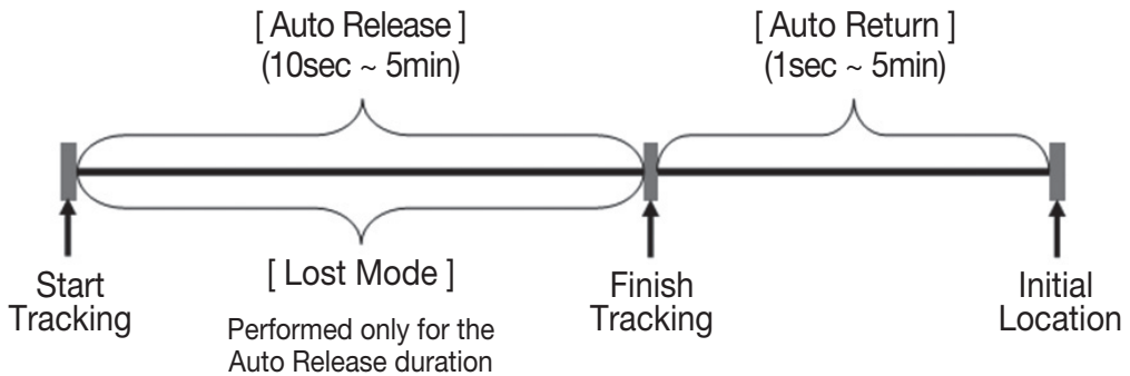
<Auto Track Timing Chart>
