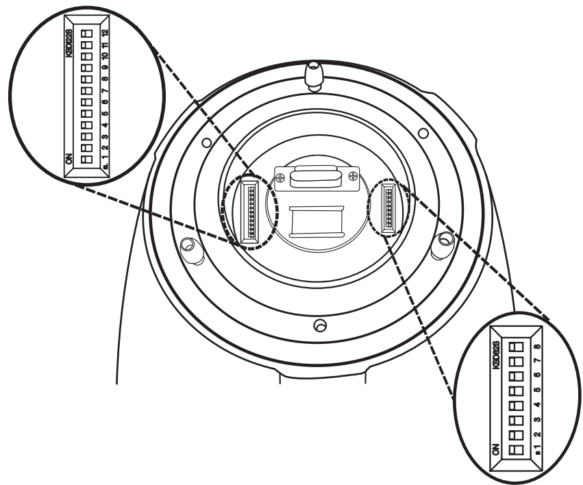
Camera ID DIP Switch(SW1)
